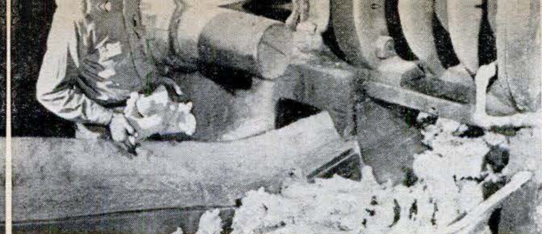
1 THIS DOUGHY MASS coming out of a Banbury mixer and dropping onto a conveyor belt is the raw beginning of asphalt tile. The ingredients, now thoroughly mixed, are a blend of asbestos, pitches, synthetic resins, pigments and limestone filler.
